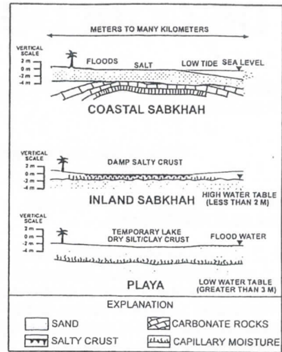
Figure 3. Idealized cross-section of sabkhas and playas, modified from Fookes (1976). Coastal sabkhas are influenced by tidal action and may be flooded during high tides. Inland sabkhas are influenced by high water tables and the capillary moisture maintaining a damp salty crust. Playas are intermittent lakes with dry silt and clay crusts.
